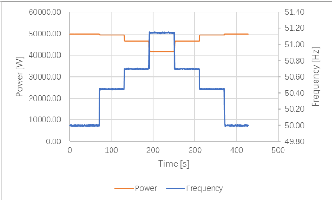
Test sequence at Registered Capacity =100%
