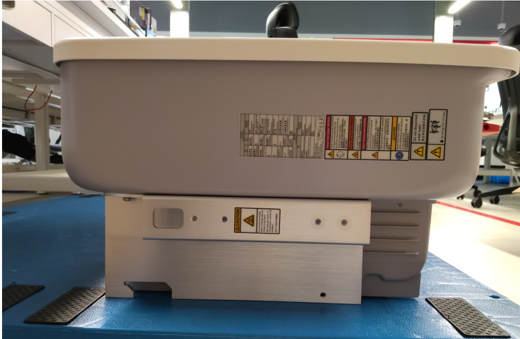
Left Side view (For models SUN2000-30KTL-M3, SUN2000-36KTL-M3, SUN2000-40KTL-M3)
