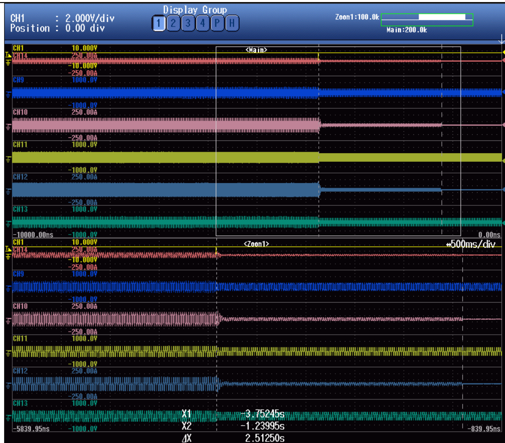
Under voltage at 184V
