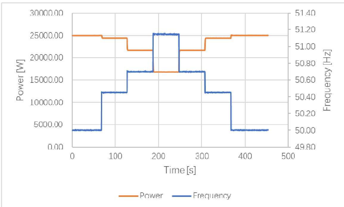
Test sequence at Registered Capacity =50%
