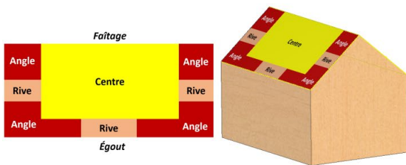
TWO-SLOPED ROOF
