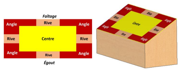
ONE-SLOPED ROOF
