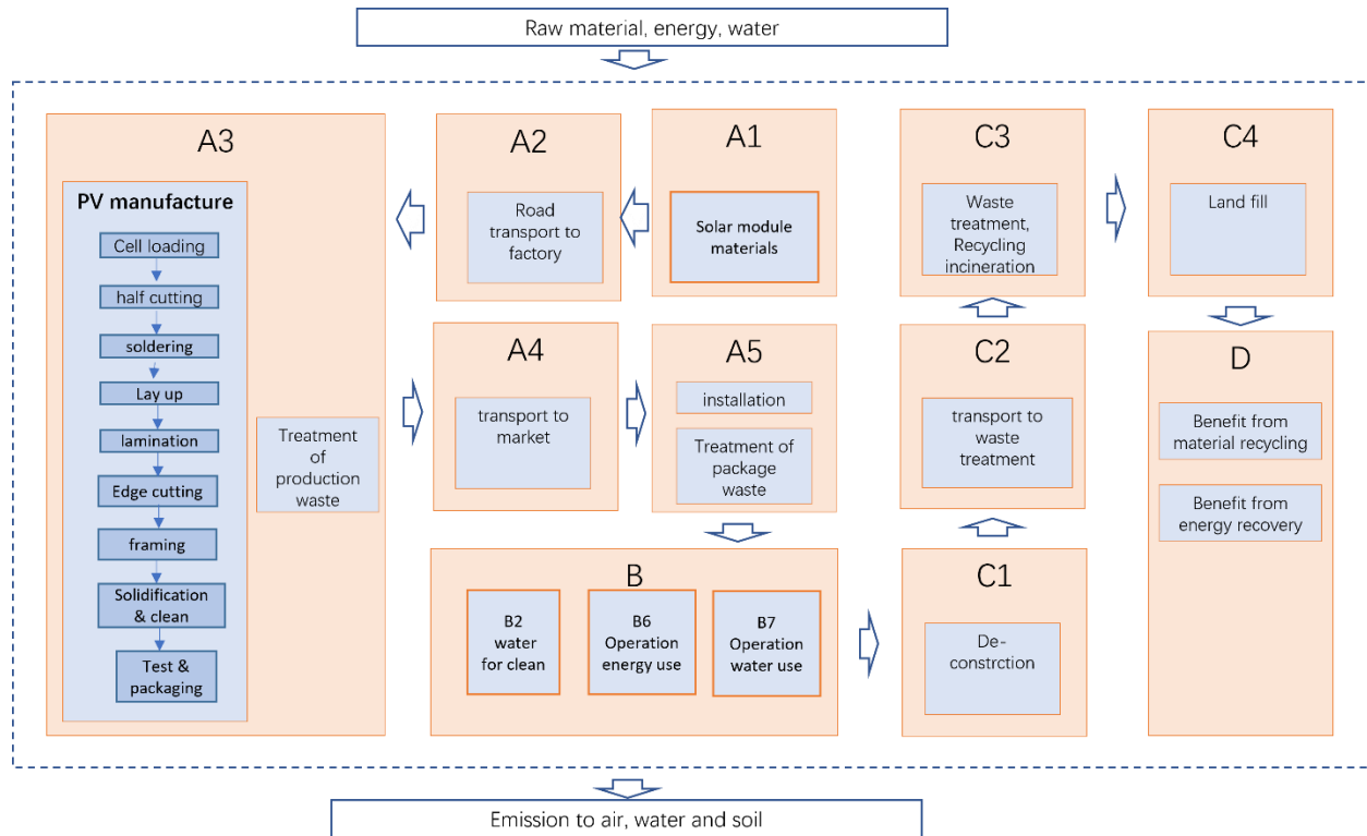
Figure 2. System diagram
