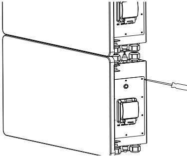
Figure 4.10 Install the right cover
