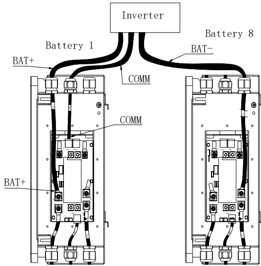
Figure 4.6 Battery to inverter wiring
