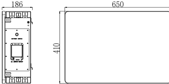
Figure 3.1 B1-5.1-48 exterior and dimension
